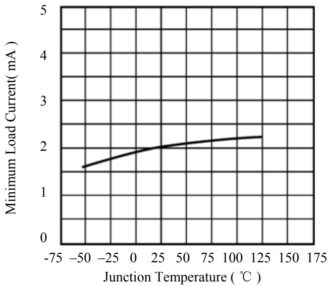
Figure 8. Minimum Load Current VS. Temperature
