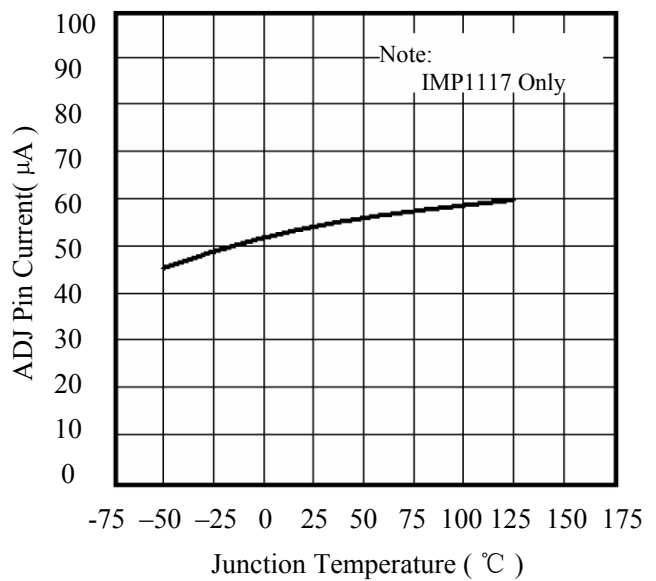
Figure 9. ADJ Pin Current VS. Temperature
