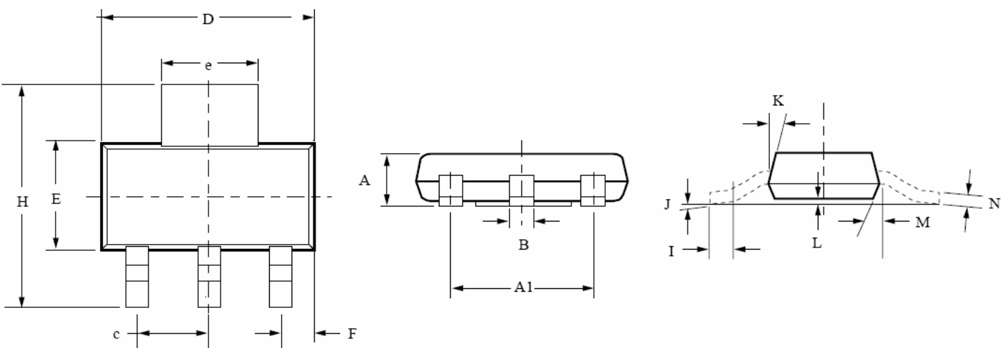
Figure 10. 4-Lead SOT-223 Package
