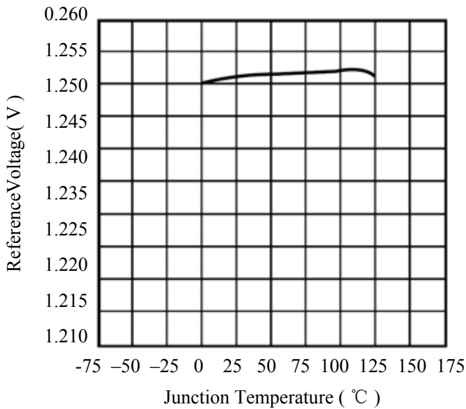
Figure 6. Reference Voltage VS. Temperature
