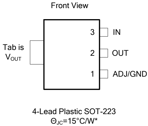
Figure 2. Pin Assignments of IMP1117
