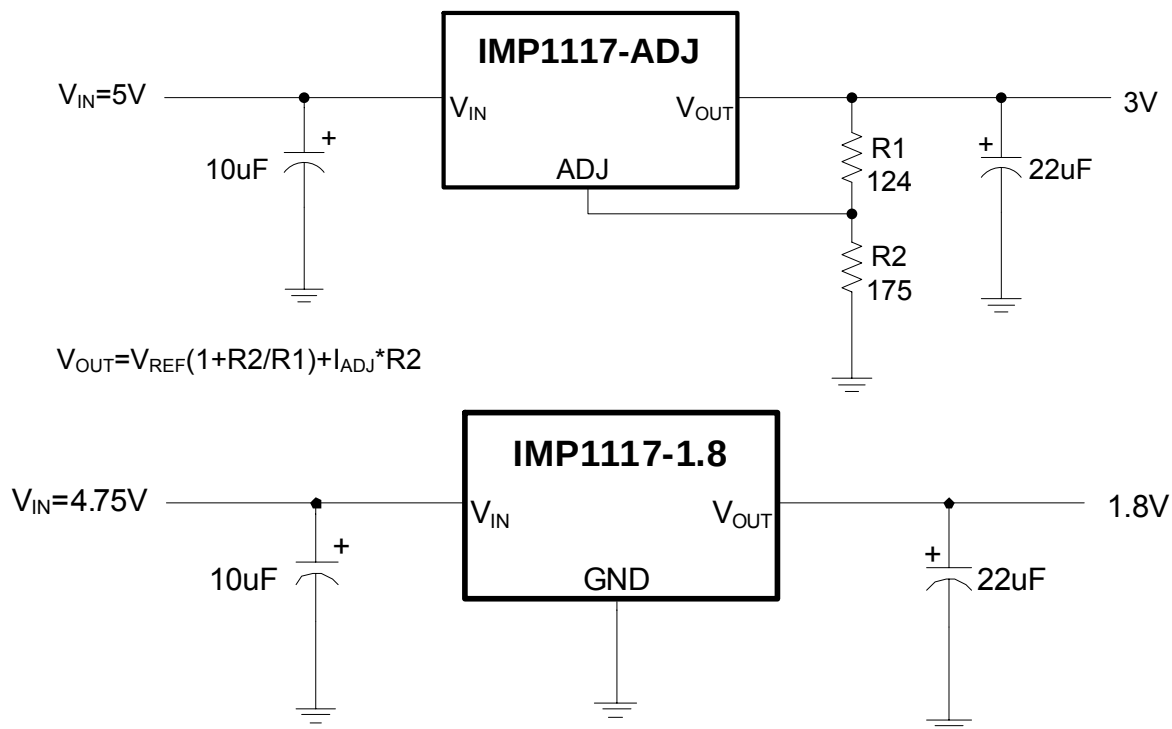
Figure 1. Typical Applications of IMP1117
