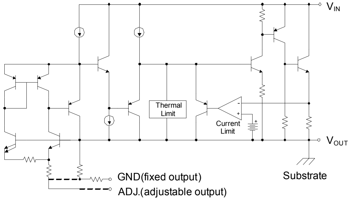
Figure 4. Block Diagram of IMP1117
