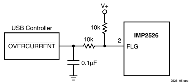
Figure 4. Transient Filter
